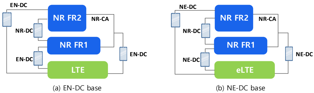
Figure 15. High-band utilization based on NSA option
