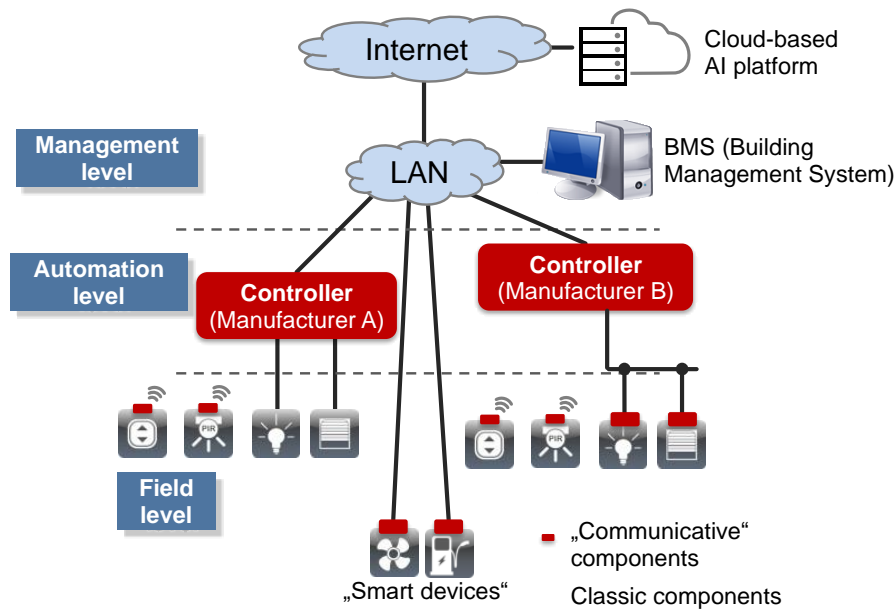
Illustration 2: linking building automation with a (cloud-based) AI platform
