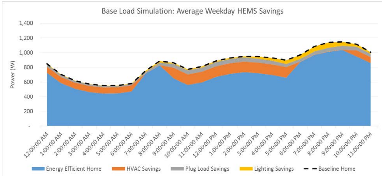
Figure 6. Base-load Simulation Model Maximum Potential Savings for Average Home on an Average Weekday
