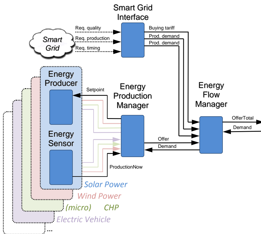
Figure 7 – Production of electrical energy and Smart Grid Interface in the KNX Energy Management model
