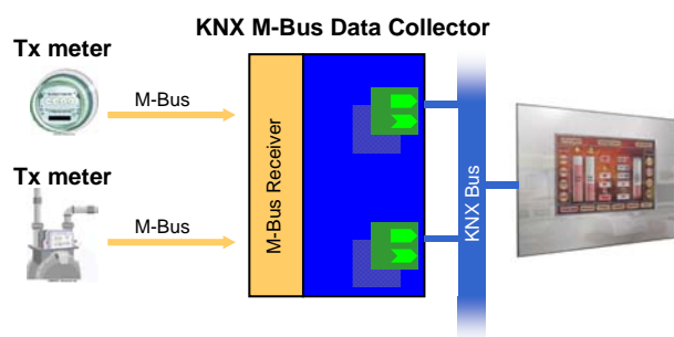
Figure 1 – The display is fed by the KNX M-Bus Meter with KNX module snapped on
