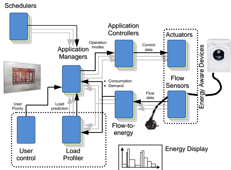
Figure 5 – Load Management with KNX (not all links are drawn)
