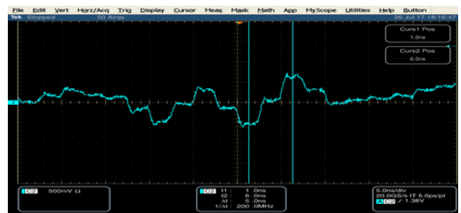
Figure 7: 6-around-1 Symbol time of Victim Pair A IEEE 802.3bz 2.5Gb/s 2m (p) + 100m (h) + 2m (p). All disturbers IEEE 802.3bz linked at 2.5Gb/s.
