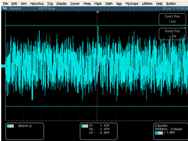
Figure 8: 6-around-1 Amplitude of Victim (Pair A) in IEEE 802.3.40 1000Base-T 6-around-1 channel 2m (p) + 100m (h) + 2m (p) amplitude. 6 disturbers comprised of 2 IEEE 802.3bz 2.5Gb/s links + 4 proprietary non-IEEE 802.3bz compliant links. Here the victim has downshifted from 2.5Gb/s to 1Gb/s after application of 4 non-compliant aggressor links.
