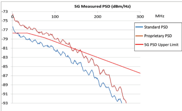
Figure 1: Measured 5Gb/s Standard-compliant vs. Proprietary non-standard compliant Transmit PSDs and IEEE 802.3bz PSD Mask [McClellan]
