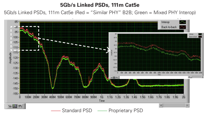
Higher Tx power is again observed in back-to-back vs. interop configurations. Total non-IEEE transmit power is estimated to be ~2 to 3 dBm higher.
