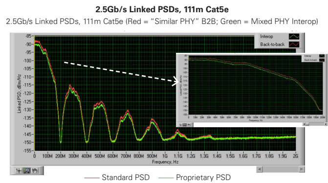
Higher Tx power is again observed in back-to-back vs. interop configurations. Total non-IEEE transmit power is estimated to be ~2 dBm higher.
