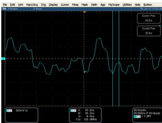
Figure 9: Symbol time of Victim (Pair A) IEEE 802.3.40 1000Base-T in 6-around-1 channel 2m (p) + 100m (h) + 2m (p) amplitude. 6 disturbers comprised of 2 IEEE 802.3bz 2.5Gb/s links + 4 proprietary non-IEEE 802.3bz compliant links. Here the victim has downshifted from 2.5Gb/s to 1Gb/s after application of 4 non-compliant aggressor links.
