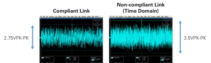
Figure 10: Amplitude of non-IEEE compliant link is much higher (3.5Vpk-pk) than the IEEE 802.3bz compliant link (2.75V pk-pk). High amplitude causes noise contamination on neighboring links.
