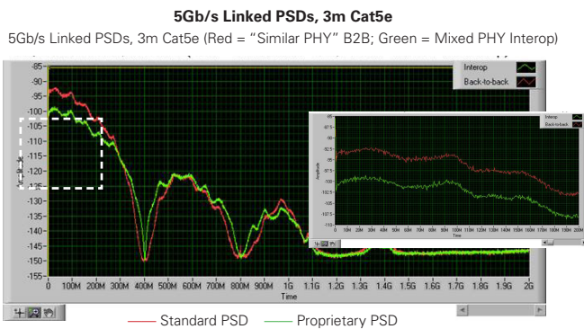
Note higher Tx power in the back-to-back (same PHY, assumed non-IEEE mode) configuration compared to the interop (different PHYs, assumed IEEE-compliant mode) configuration. Total non-IEEE transmit power is estimated to be ~6dBm higher.
