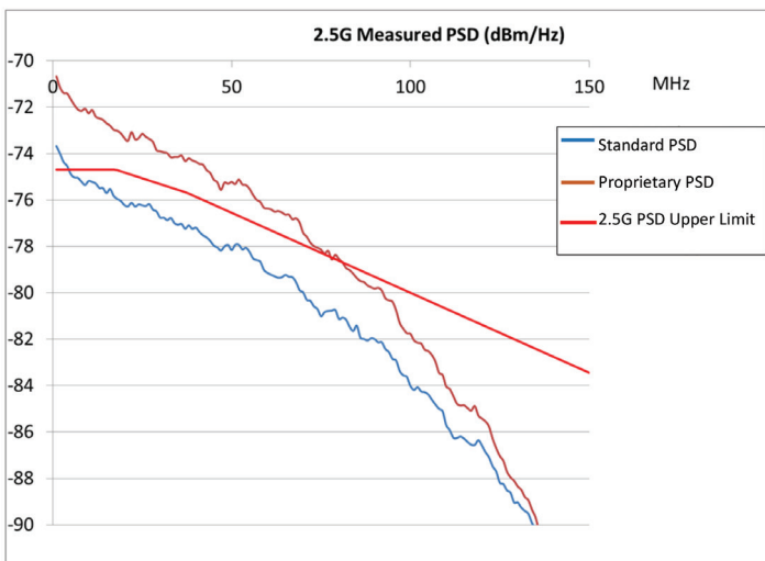
Figure 2: Measured 2.5Gb/s Standard-compliant vs. Proprietary non-standard compliant Transmit PSDs and IEEE 802.3bz PSD Mask [McClellan]
