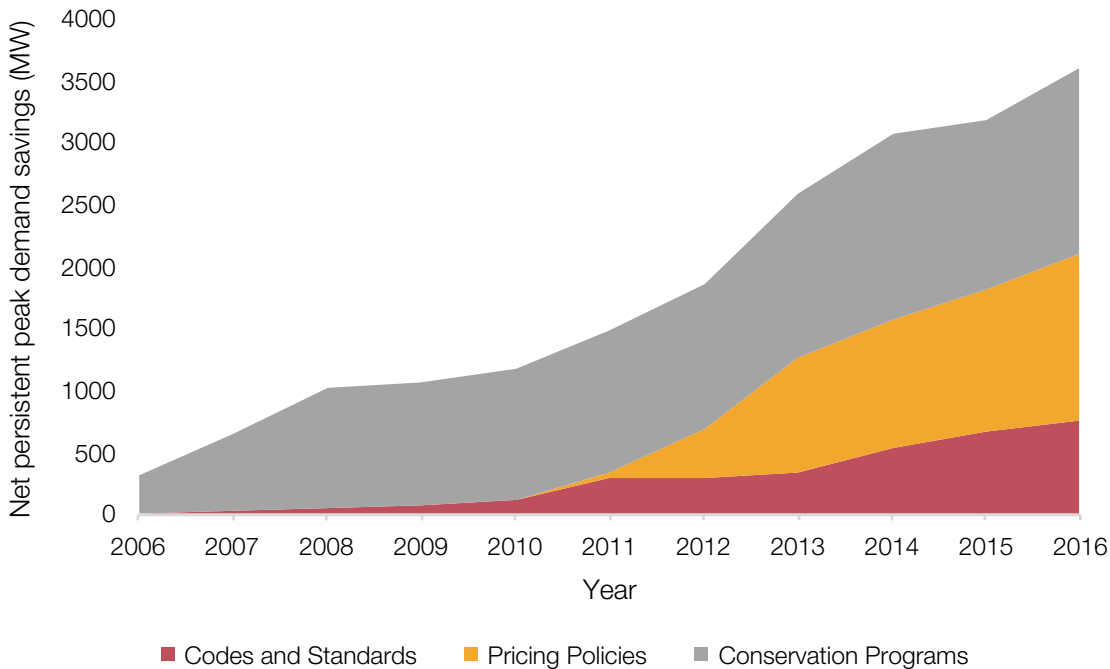
Figure 3.9. Net persisting peak demand savings, 2006-2016 (Ontario).
