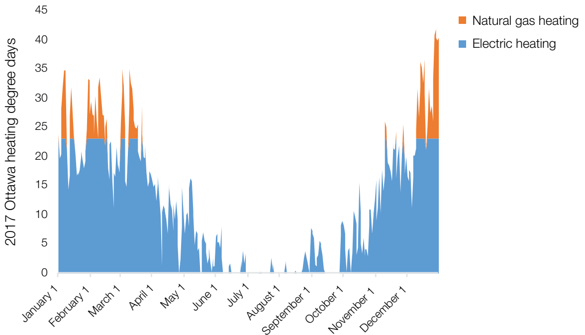
Figure 15.7. Electric and natural gas heating systems can work together to reduce the costs of emission reductions.
