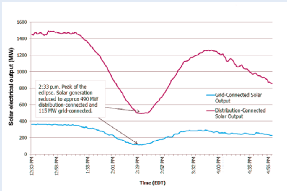
Figure 6.7. Change in solar generation output on 21 August 2017.
