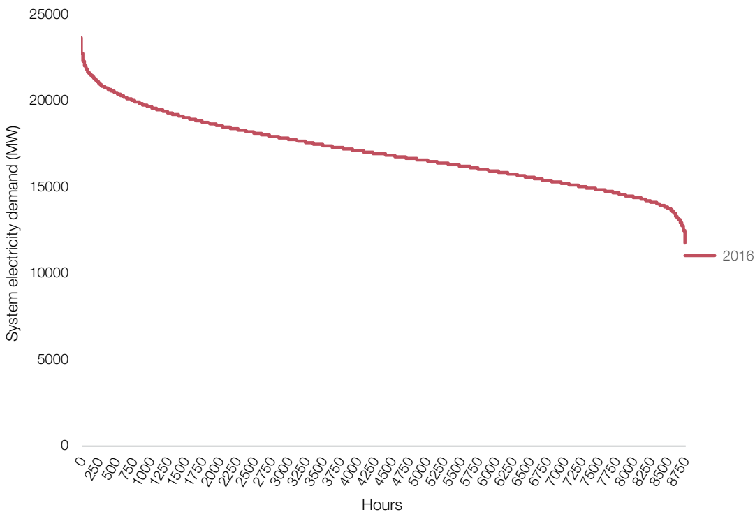
Figure 3.4. The range of electricity demand in Ontario (2016) (i.e., the load duration curve).
