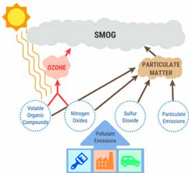
Figure 12.2. How smog forms in the atmosphere.
