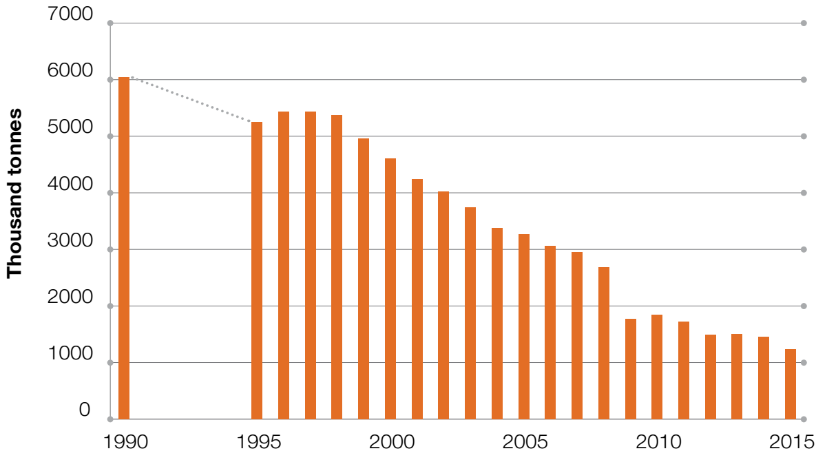
Figure 12.9. NO x emission trends from electric utilities in the U.S.
