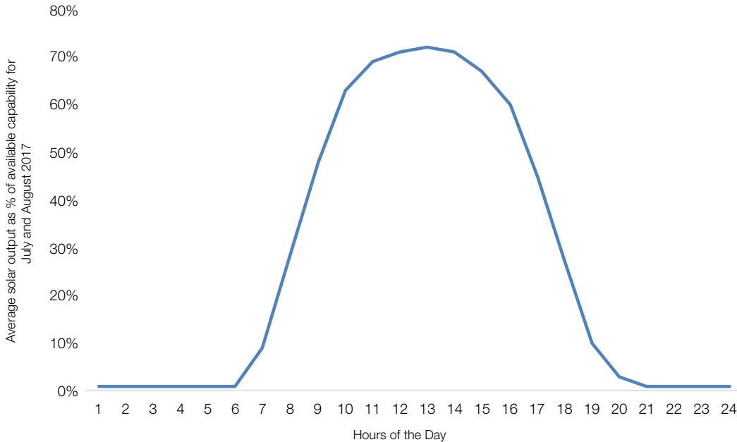
Figure 6.1. Average variation in solar electricity output over the day for July and August 2017.
