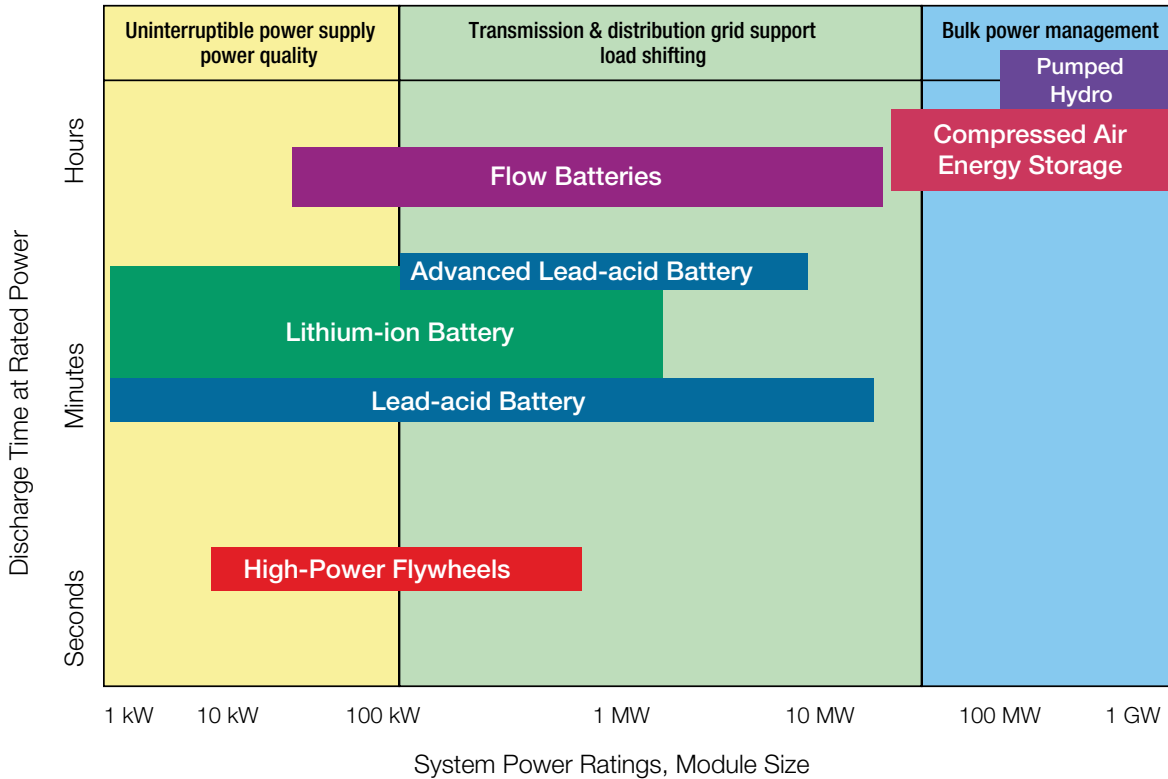
Figure 16.6. Energy storage technologies per their power rating and discharge times at rated power.
