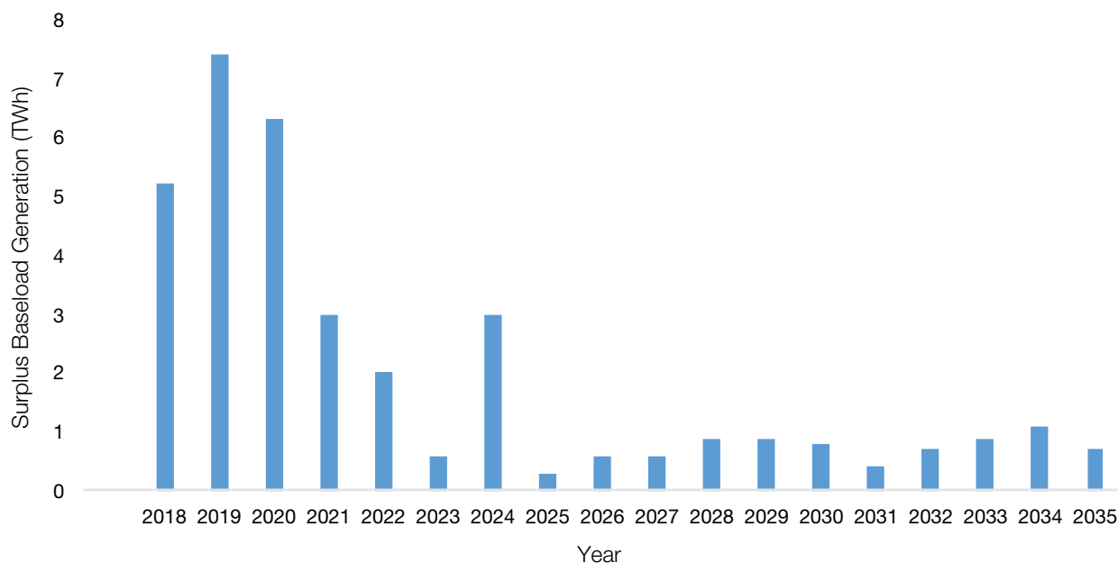
Figure 16.1. Projected curtailment of Ontario surplus electricity, 2018-2035.
