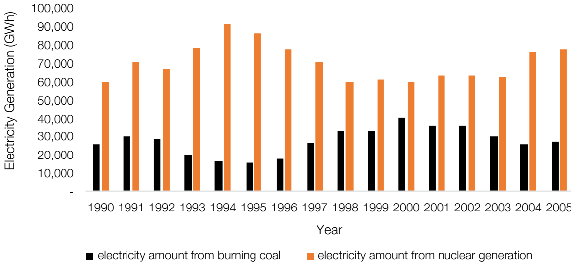
Figure 12.1. Electricity production from coal vs. nuclear-fired generating stations in Ontario 1990 - 2005.
