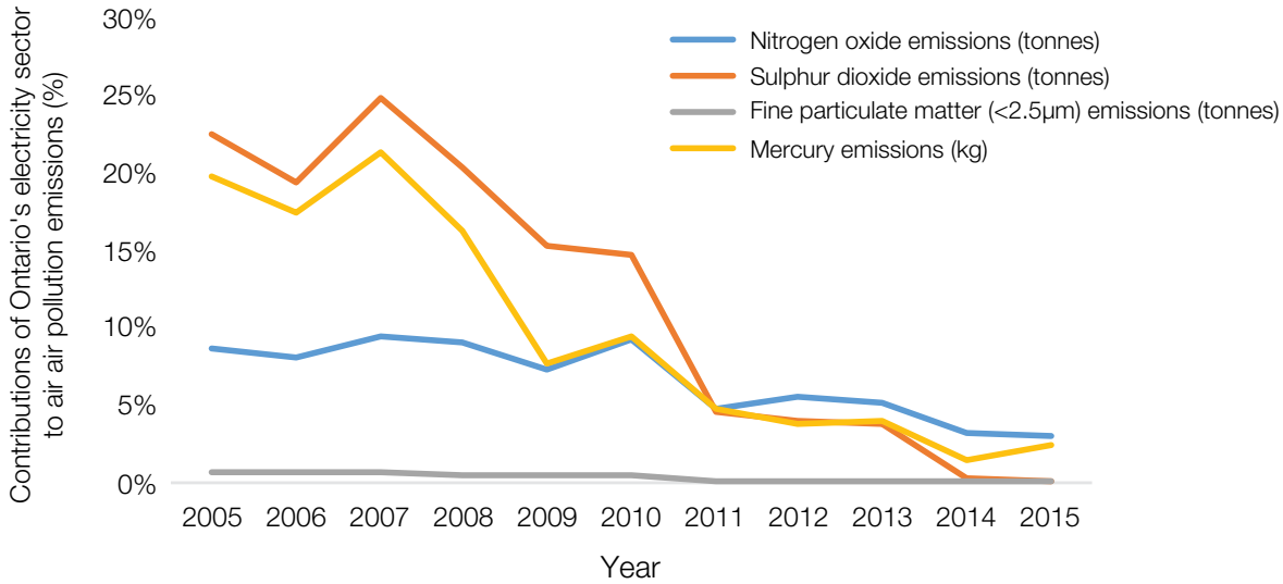
Figure 12.7. Ontario's electricity sector's contribution to Ontario's overall air pollution burden as measured with selected pollutants (2005-2015).
