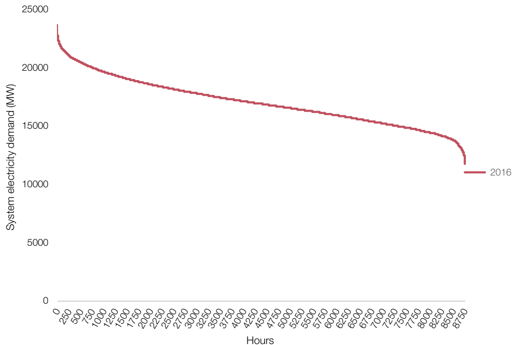
Figure 5.1. The range of electricity demand by hour, or 'load duration curve', for 2016 (Ontario).
