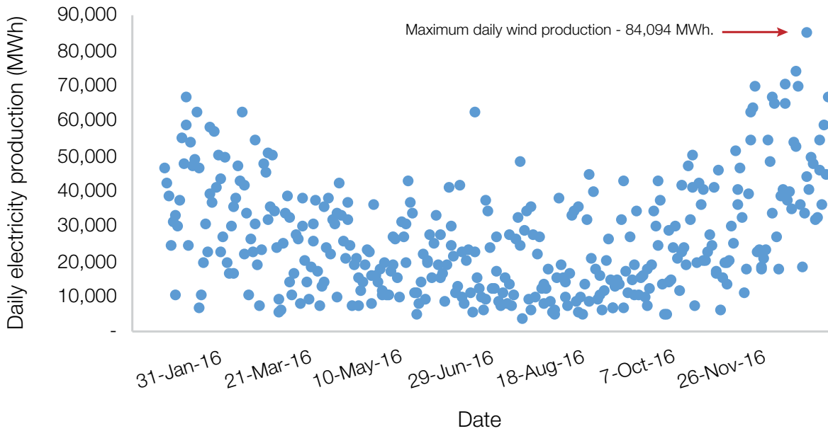
Figure 6.3. Variation in daily Ontario wind production throughout 2016.
