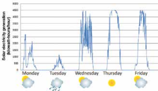
Figure 6.2. Variability of solar output depends on local weather conditions – an example from the Princeton University Solar Field April 11-16, 2013.
