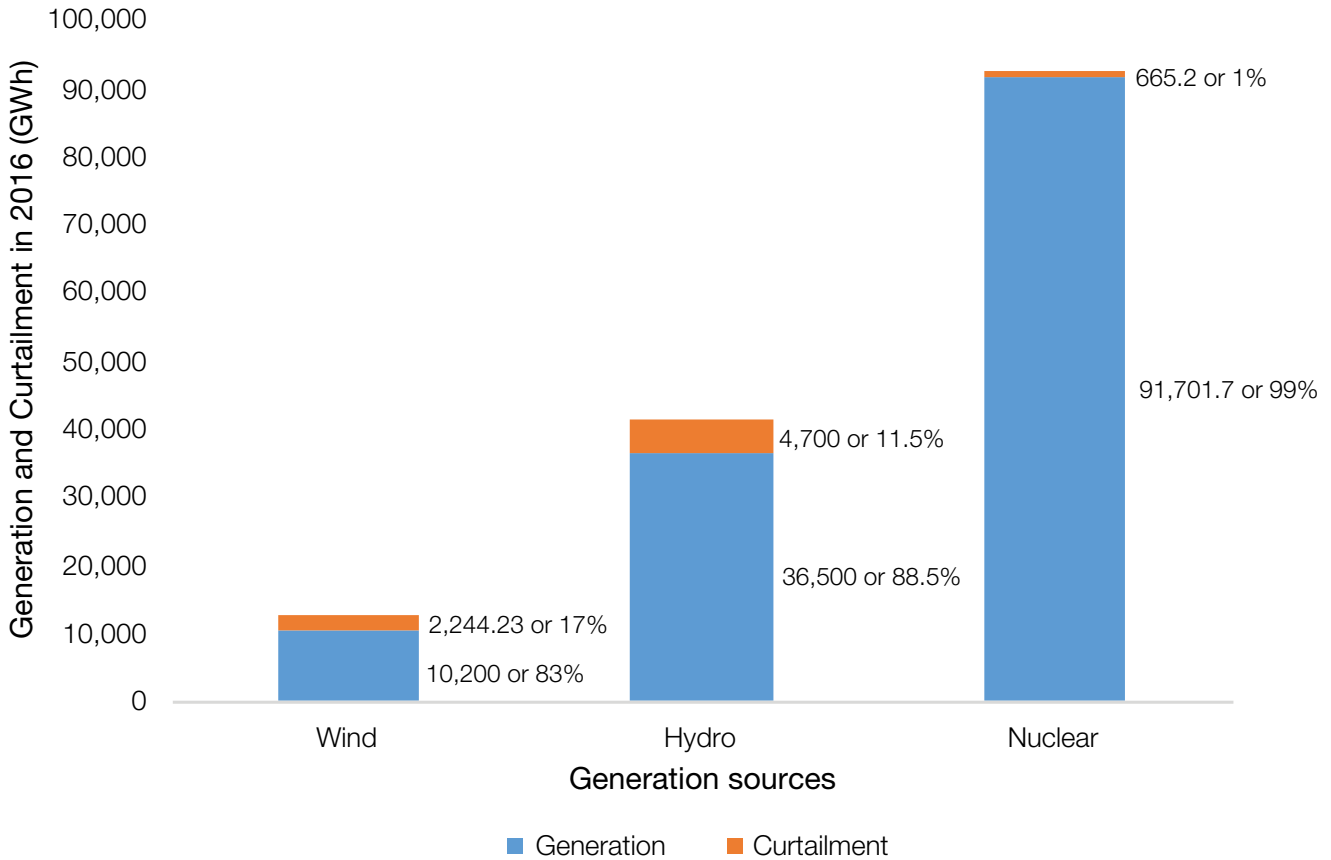
Figure 7.9. Curtailment as a share of Ontario’s grid-connected production for wind, hydro and nuclear generation in 2016.
