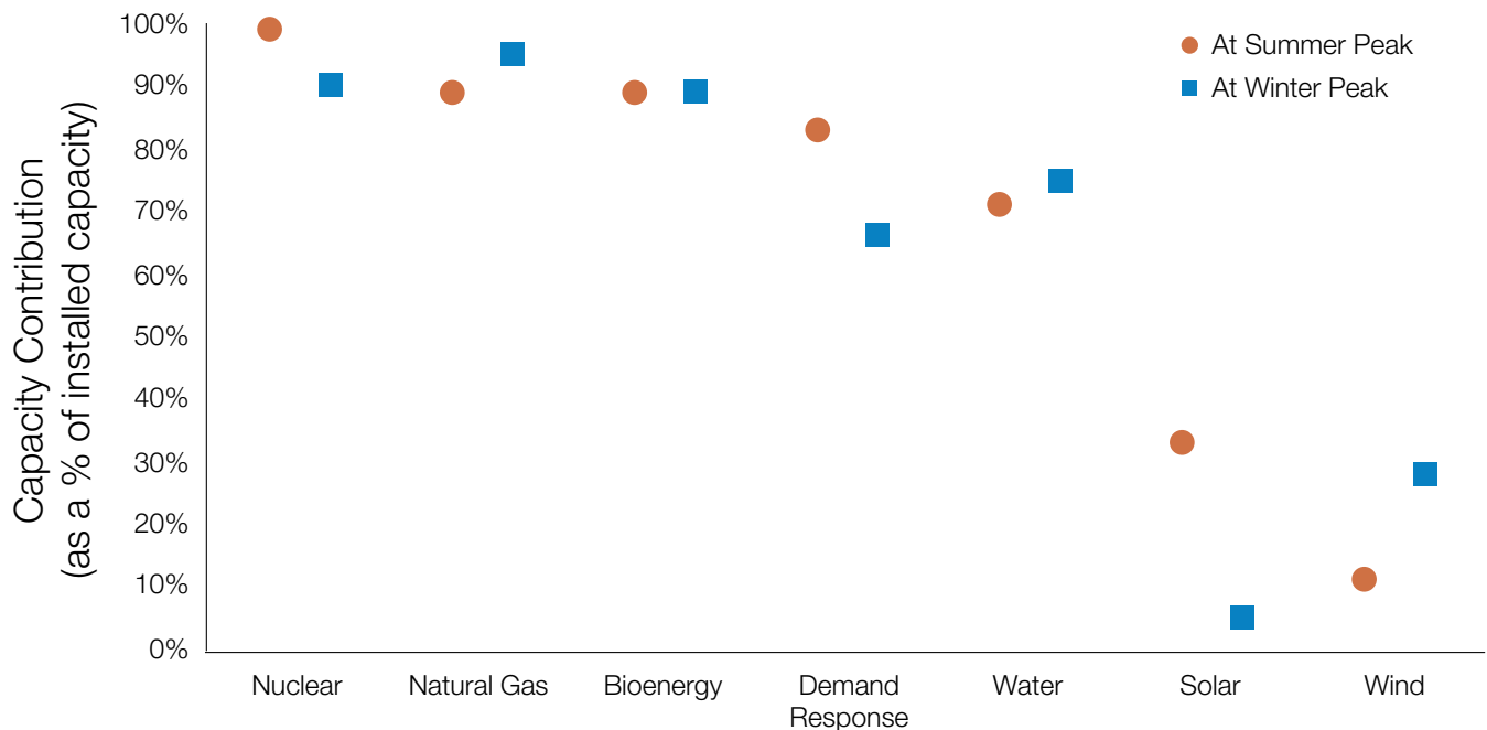
Figure 5.3. Peak demand capacity contribution (summer vs. winter, Ontario).
