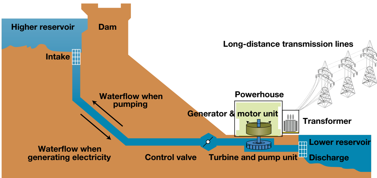
Figure 16.5. Schematic of a typical pumped hydro storage system.
