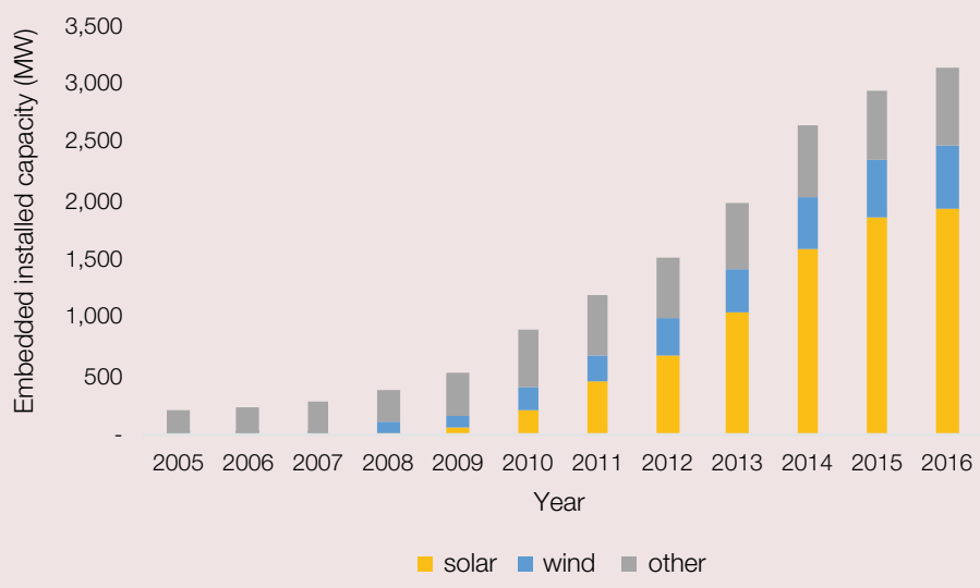
Figure 4.10. Ontario’s embedded installed capacity at year end.
