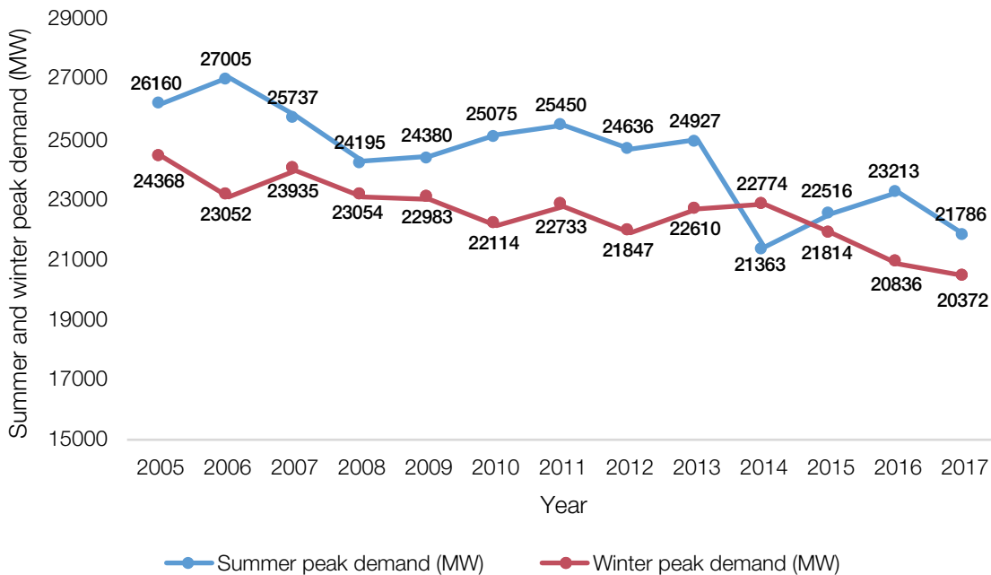
Figure 3.5. Historical annual peak demand, summer and winter, 2005-2017.
