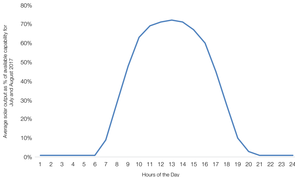
Figure 5.4. Average variation in solar electricity output over the day for July and August 2017.
