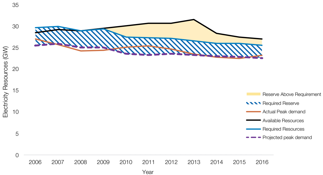
Figure 5.5. Comparison of Ontario's projected vs. actual peak demand with available resources, 2006-2016.
