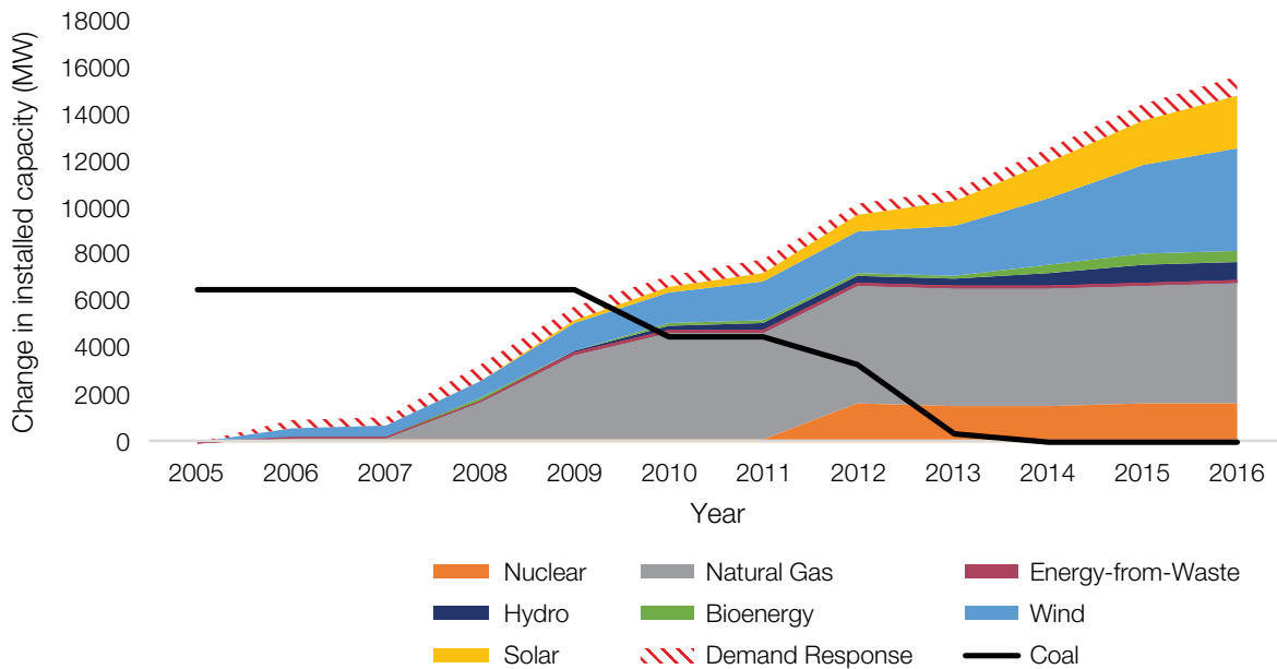
Figure 4.3. Net change in Ontario’s installed capacity (grid connected and embedded), by generation type, 2005-2016.
