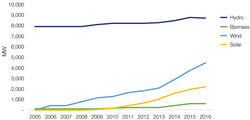
Figure 4.6. Total renewable electricity capacity in service by energy source.
