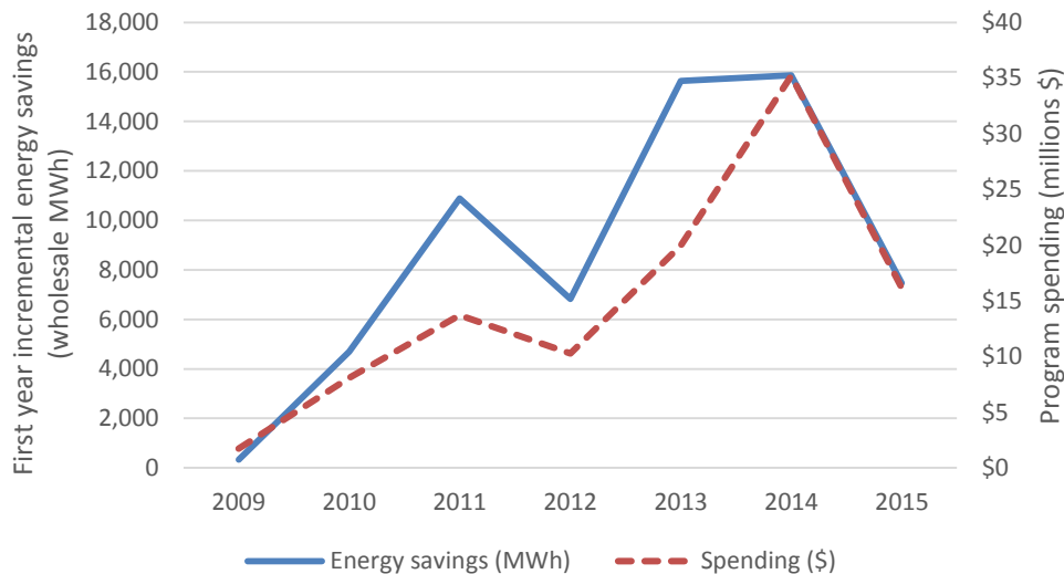
Figure 5. Limited-income program spending and first-year savings, 2009–2015
